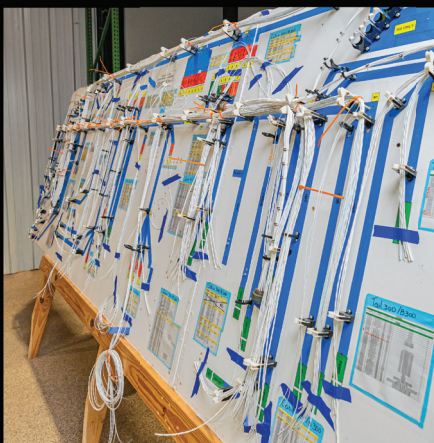
Connector and Wire Harness Assembly
